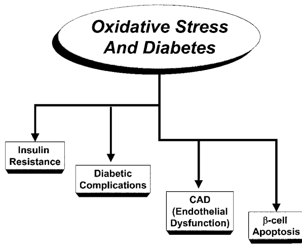
FIG. 6. Potential areas of impact of oxidative stress in diabetes and the pre-diabetic state. Free radical generation leading to oxidative stress has the capacity to impact diabetes at multiple levels. The role of oxidative stress leading to microvascular complications has the most experimental support. Oxidative stress also plays a significant role in the development of macrovascular complications, including promoting atherosclerosis and the inhibition of nitric oxide-mediated vasodilation. 21 More recent evidence suggests an association of oxidative stress with both impaired insulin action ( in vitro and in vivo ) and the deterioration of \beta -cell function.
